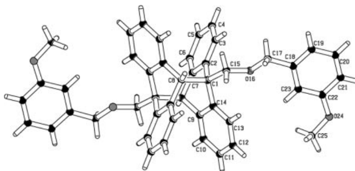
Figure 2. Crystal structure of dimer 5a (atom numbering not in accord with nomenclature rules).
