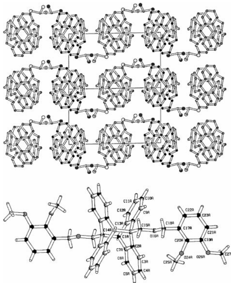
Figure 3. Crystal structure of dimer 5b . Upper part: Unit cell which contains two molecules 5b (A,B) in slightly different positions which are separated by two molecules \text{CHCl}_3 . Lower part: Platon plot of 5b (A). (atom numbering not in accord with nomenclature rules).
