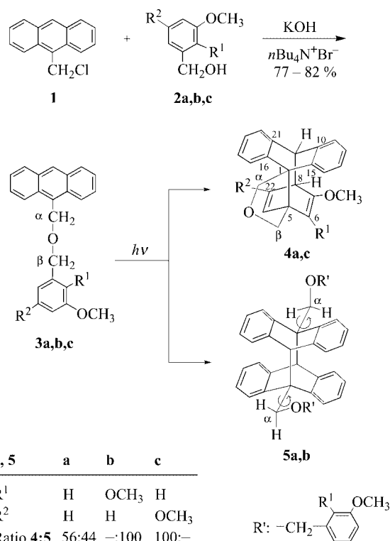
Scheme 1. Preparation and photoreactivity of 9-[(arylmethoxy)methyl]anthracenes ( 3 ).
