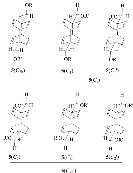
Scheme 2. Rotamers of 5 (formula without condensed benzene rings).
