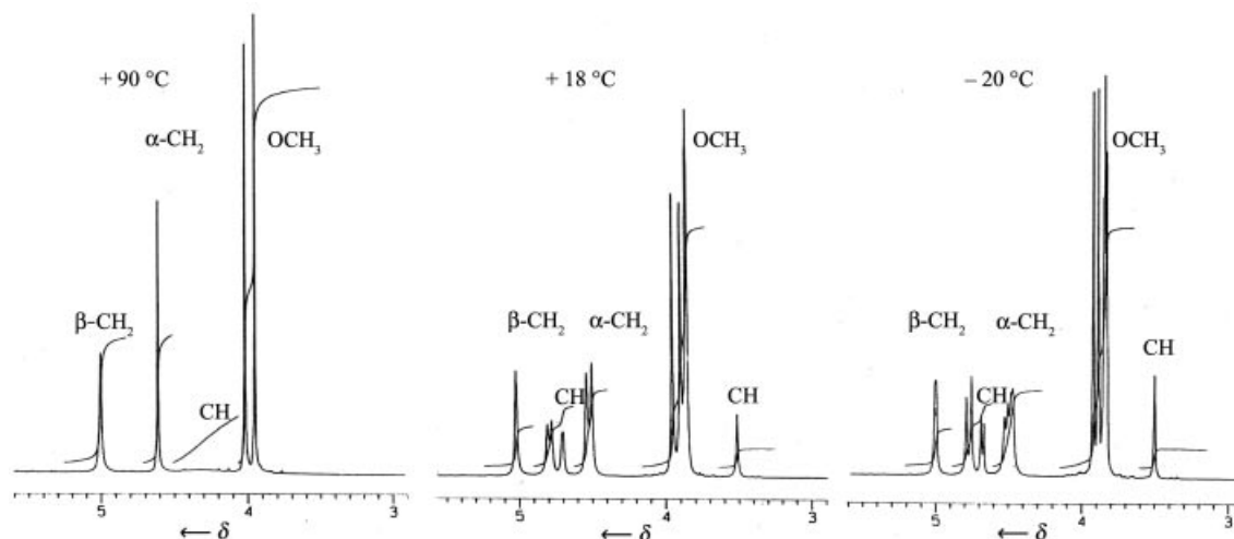
Figure 1. Temperature-dependent ^1\text{H} -NMR spectra (in the range 5.5 < \delta < 3.0 ) of 5b measured at 400 MHz in \text{CDCl}_2\text{-CDCl}_2 .
